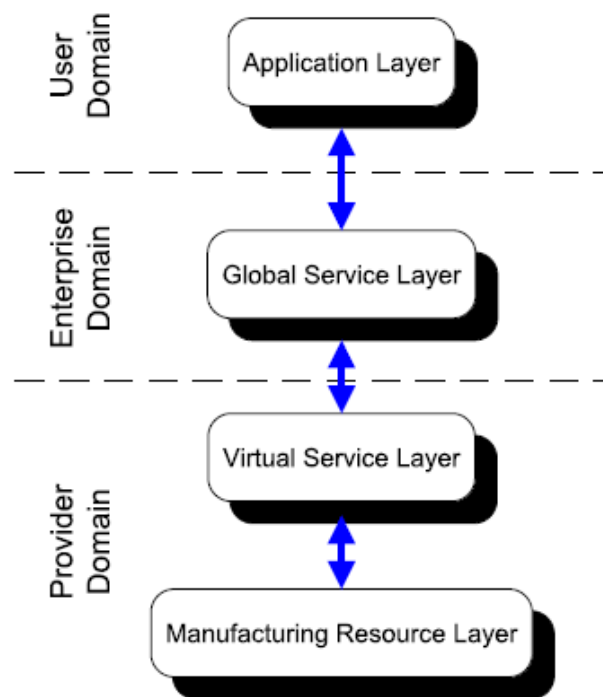
FIGURE 2: LAYERED ARCHITECTURE OF A CLOUD MANUFACTURING SYSTEM [7].
